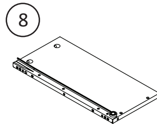
x6 T6228013080PK RIGHT DRAWER SIDE
