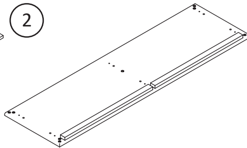
x1 T6228013020PK BOTTOM PANEL
